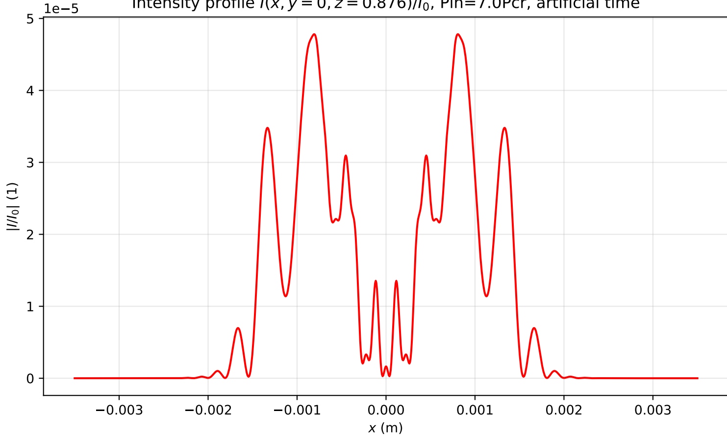
Intensity profile I(x, y = 0, z = 0.876)/I_0 , P_{in}=7.0P_{cr} , artificial time
